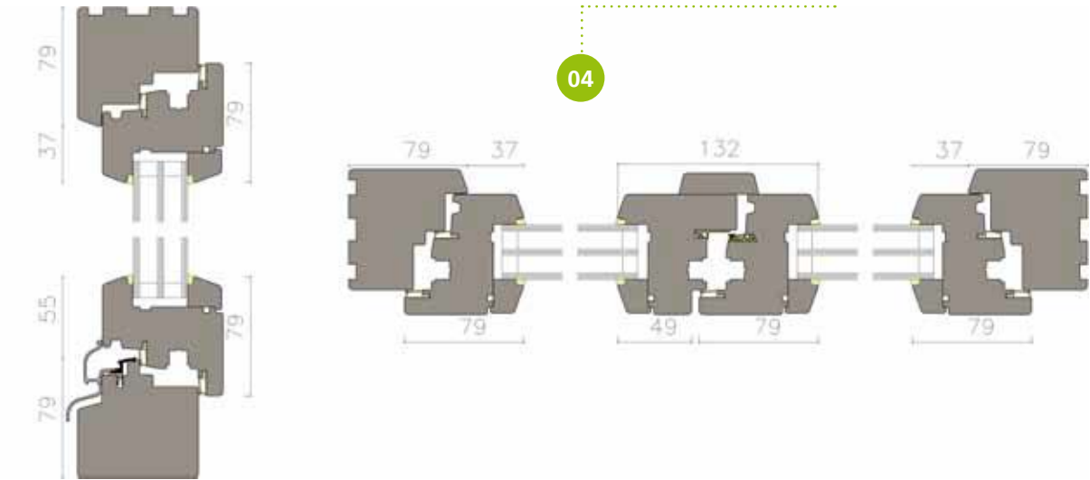
IV80 Standard 2-flügelig
